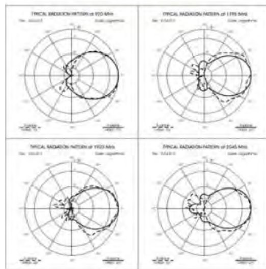
Polar diagrams for the SA918 directional antenna
